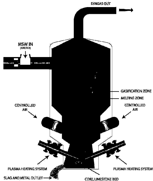
Figure 11 - Cross-Section of a Plasma Arc Furnace 12
