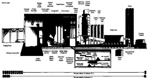
Figure 2 - Typical Mass-Burn Waterwall System 3
