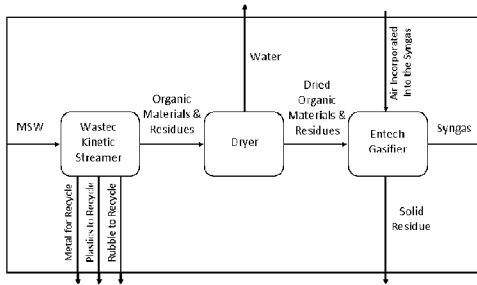
Figure 9 - EnTech Process Schematic 10
