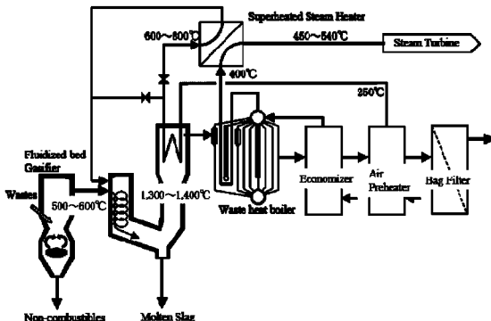
Figure 8 – RDF Fluidized Bed Gasification System 9
