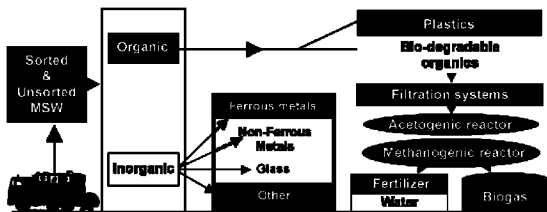
Figure 13 - Process Flow for Anaerobic Digestion System 17
