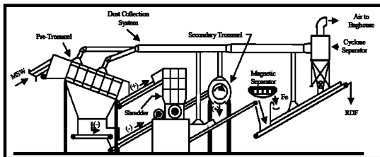
Figure 5 - Typical RDF Processing Schematic 6
